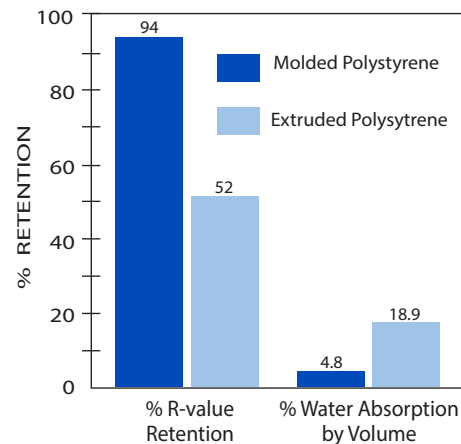
WATER ABSORPTION AND R-VALUE RETENTION 1
